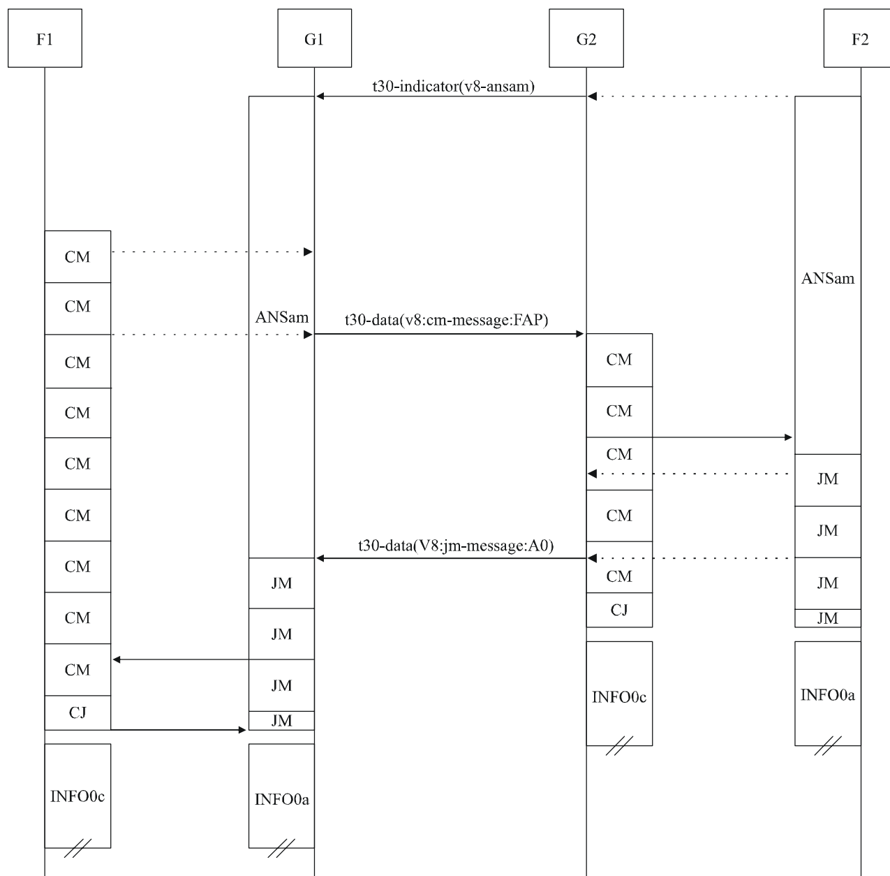
Figure IV.1 – V.8 signalling (using profiles and acks)
