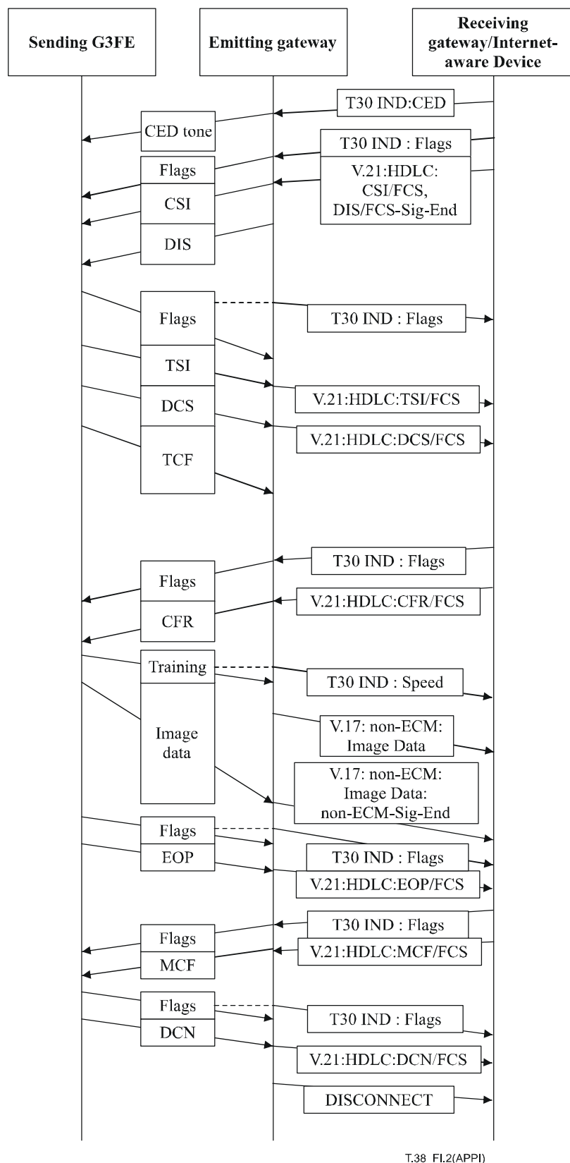
Figure I.2 – Traditional facsimile device and Internet-aware device
