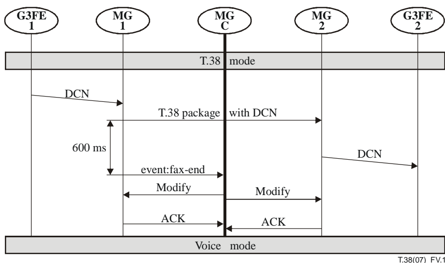
Figure V.1 – MG1 uses timer before initiating mode transition request
