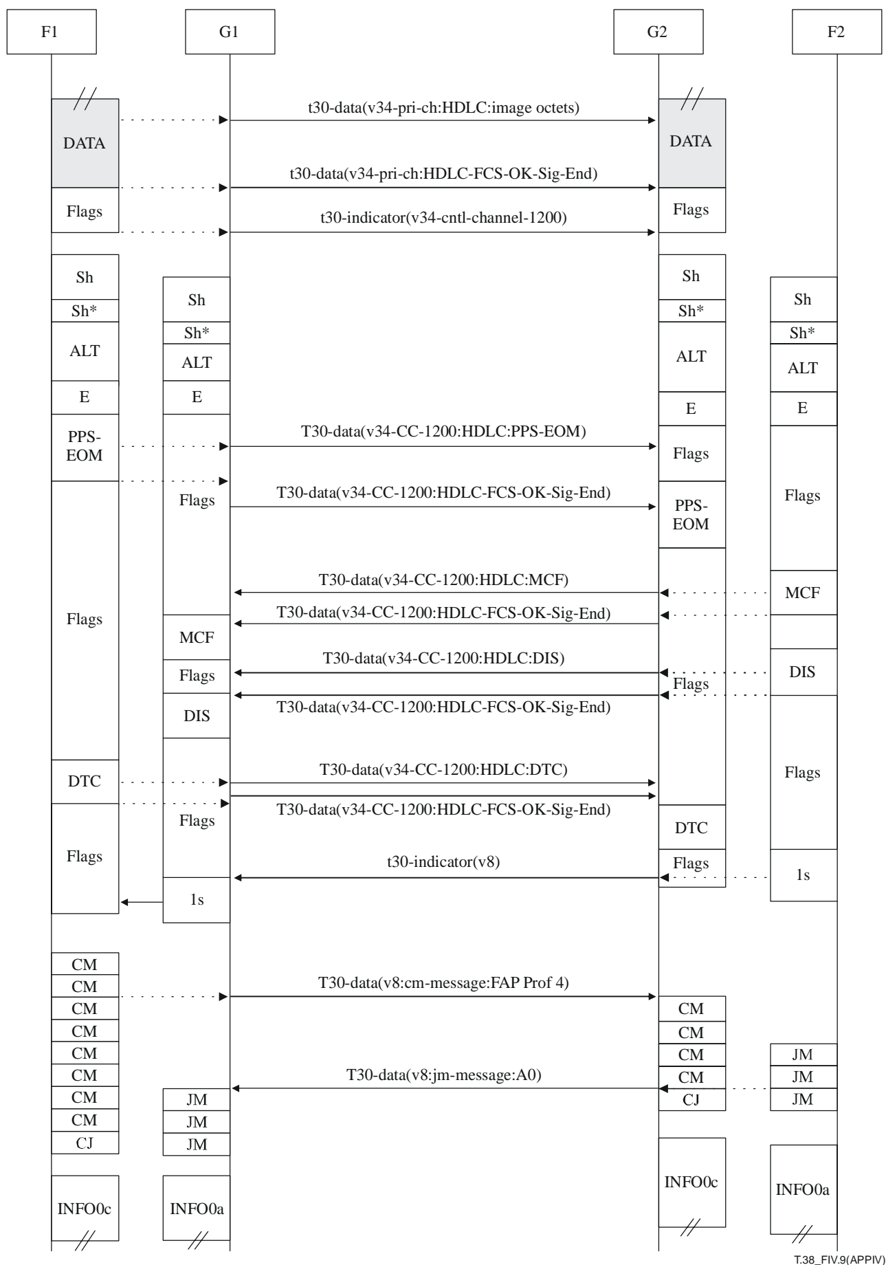
Figure IV.9 – Turn-around polling
