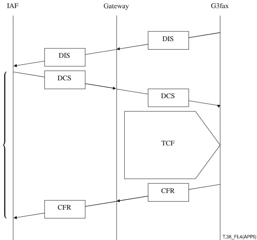
Figure I.4 – IAF transmit timing from DCS to CFR
