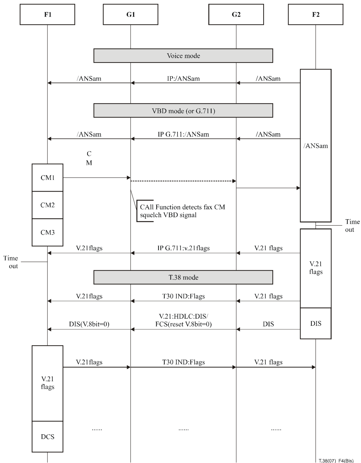
Figure F.4 – T.38 FoIP (MoIP fallback and transition to T.30 fax by Payload)
