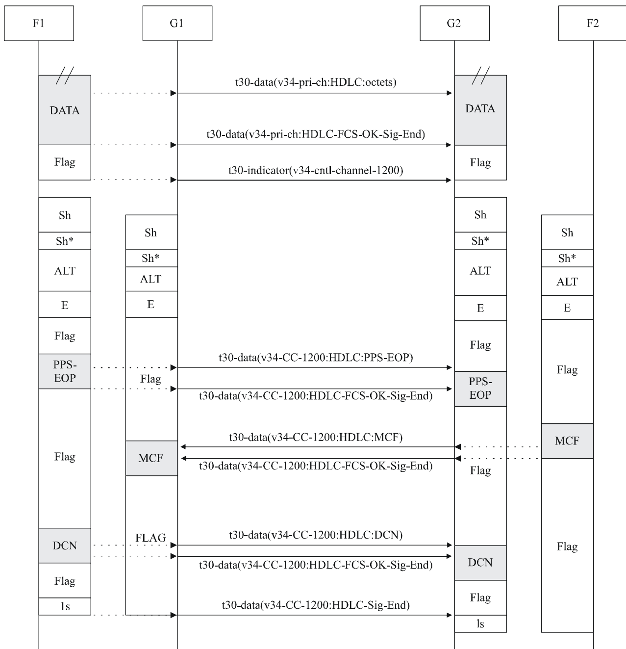
Figure IV.4 – Last page
